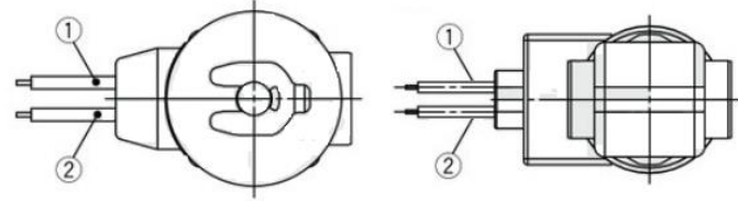
Figure 3. Grommet and grommet with PCB
