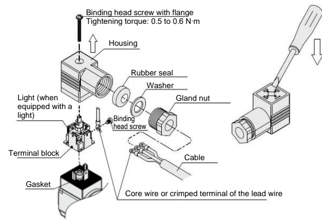
Figure 5. JSX20/30 DIN connector construction
