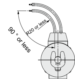
Figure 2. Lead wire bending
